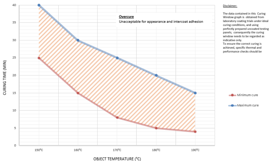
Interpon D2525 Low- E Texture- curing window
